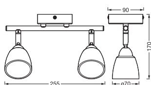
LED SPOT CUP 2XG9
