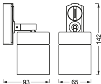
PGTRACKLIGHT SPOT CYLINDER GD WT GU10MiPRCmnk
