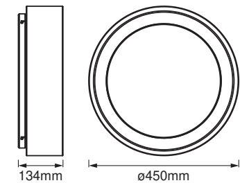
SMART WIFI ORBIS CYLNR RD 450 TW
