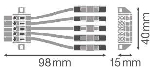
TRUSYS FLEX FEED IN CONNECTOR 5P
