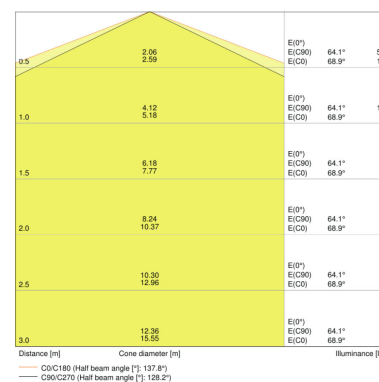
O BOLLARD 500 LANTERN 12 W 3000 K IP54 GY
