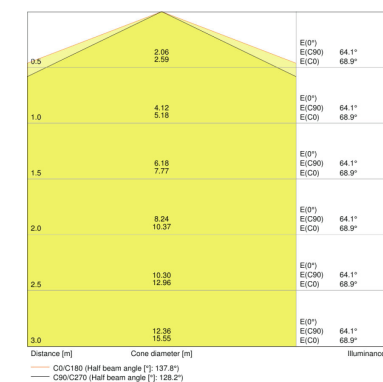
O BOLLARD 900 LANTERN 12 W 3000 K IP54 GY
