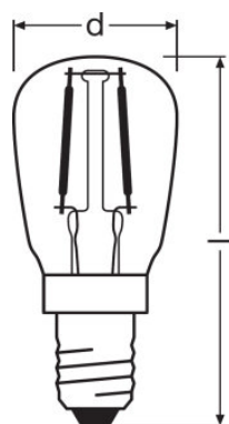
ST SPC.T26 12 2.2 W/2700K E14
