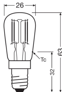
ST SPC.T26 25 2.8 W/2700K E14, ST SPC.T26 25 2.8 W/6500K E14
